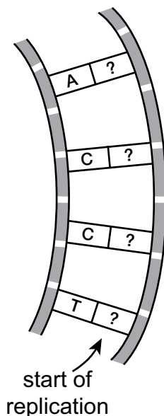
DNA Replication
