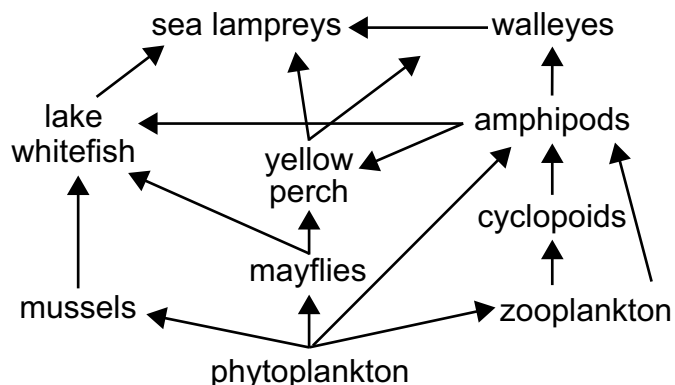
Food Web
